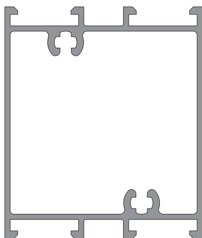
6218 1,150 Kg/m
