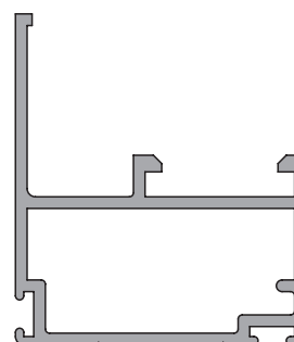
6900 0.551 kg/m
